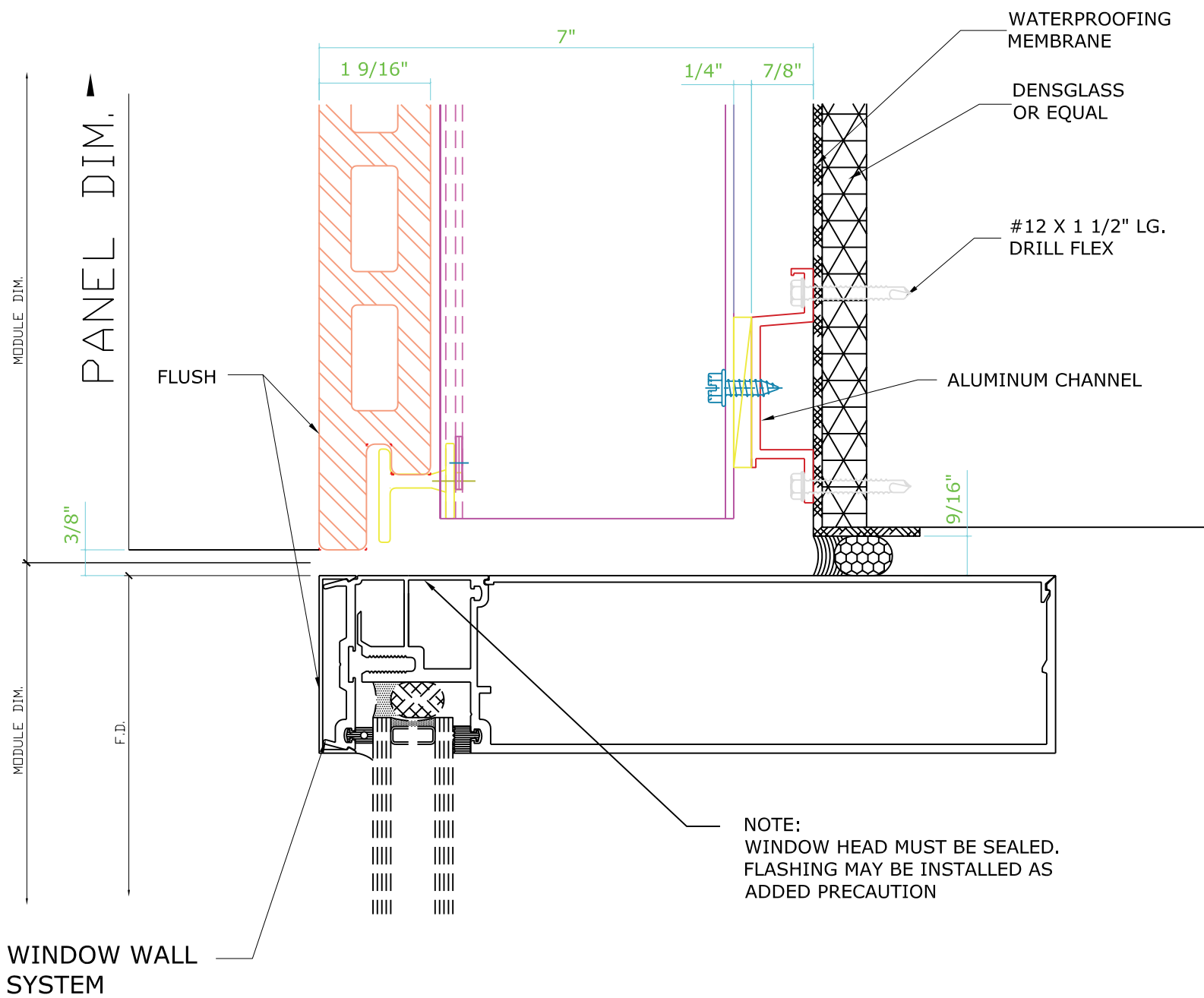
D Window Head Lrg Scale: 6"=1'
