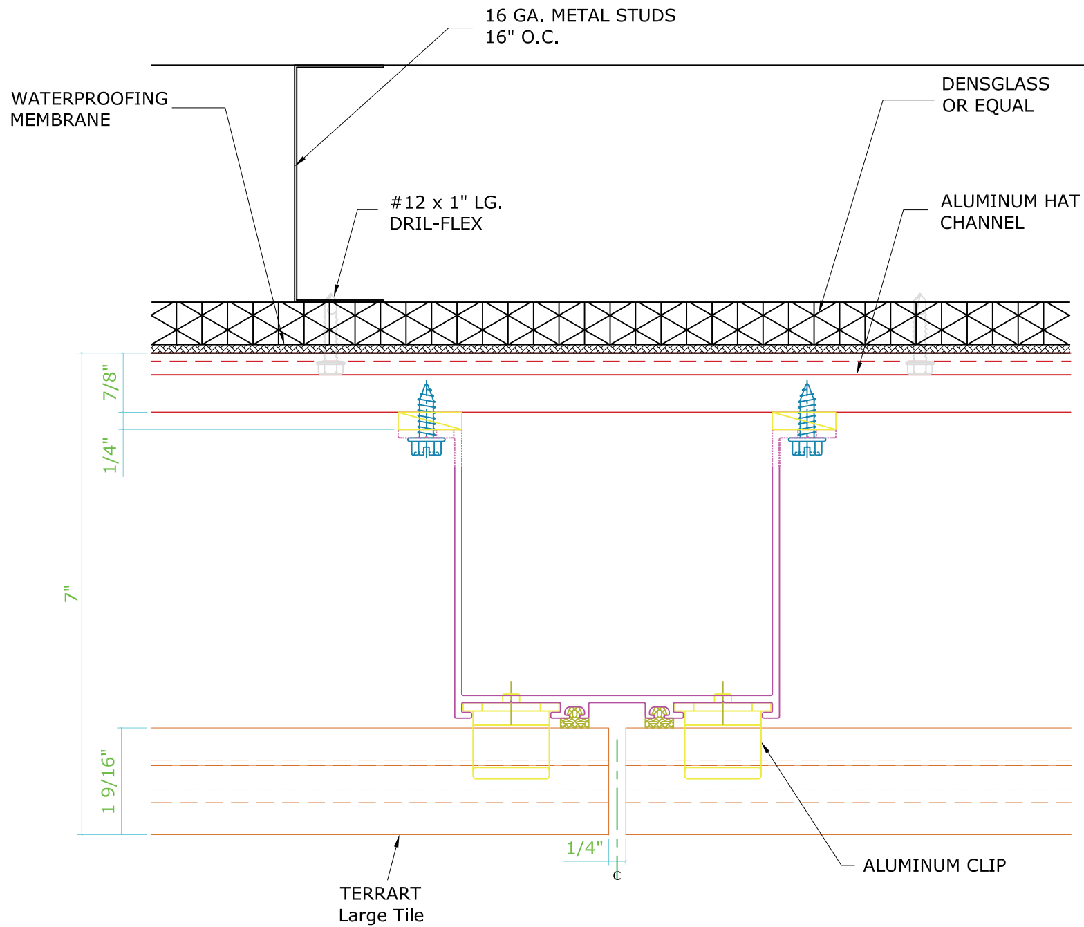
B Vertical Panel Joint Lrg Scale: 6"=1'
