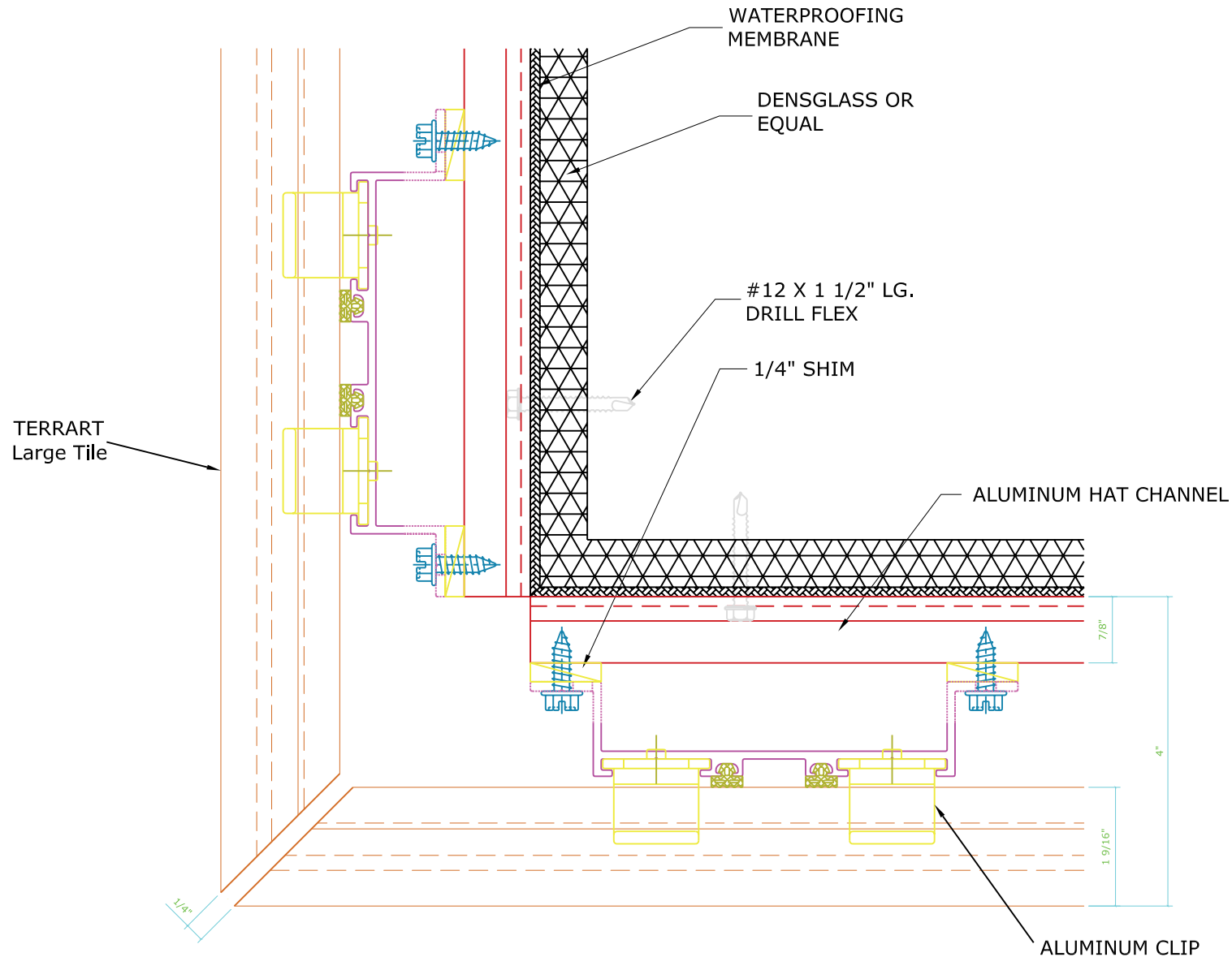
C Outside Corner Lrg Scale: 6"=1'
