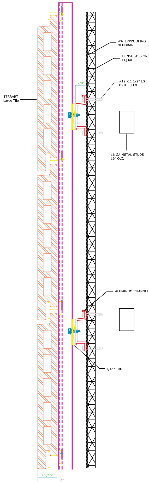
A Horizontal Panel Joint Lrg Scale: 3"=1'
