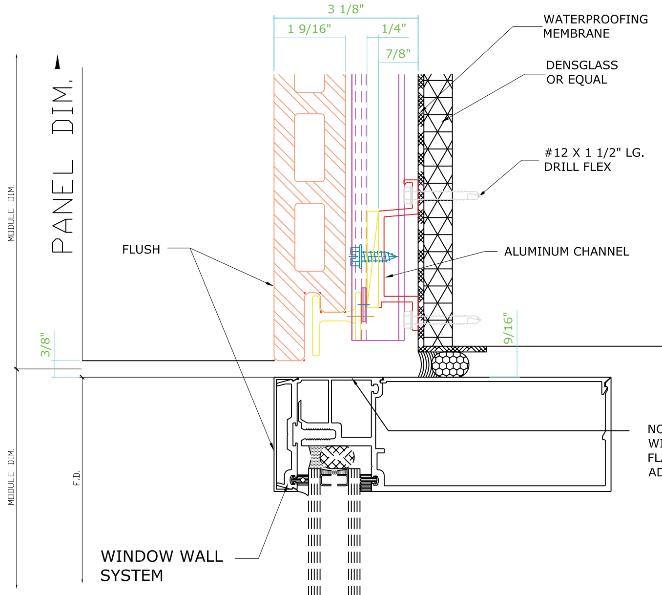
D Window Head Lrg Scale: 6"=1'
