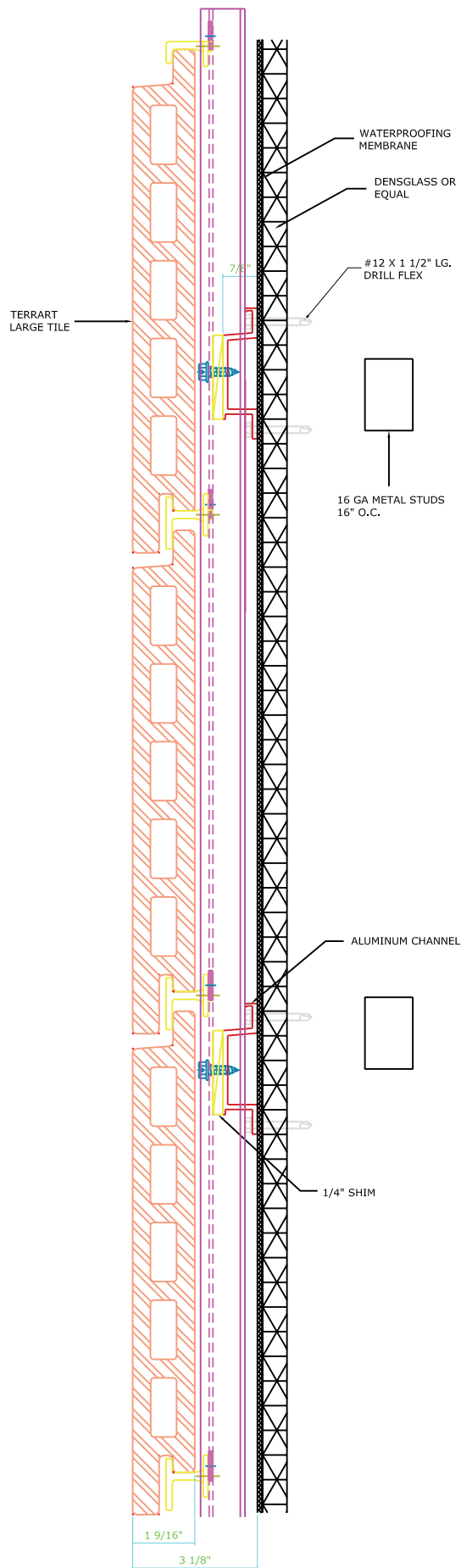
A Horizontal Panel Joint Lrg Scale: 3"=1'
